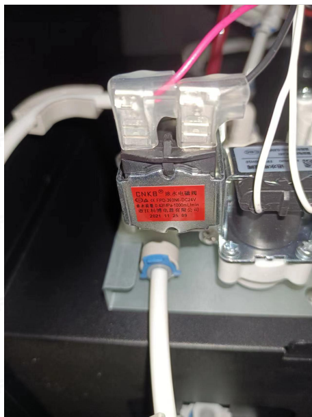
浓水电磁阀
